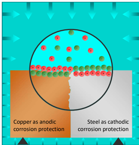
Figure 38: Functional principle
