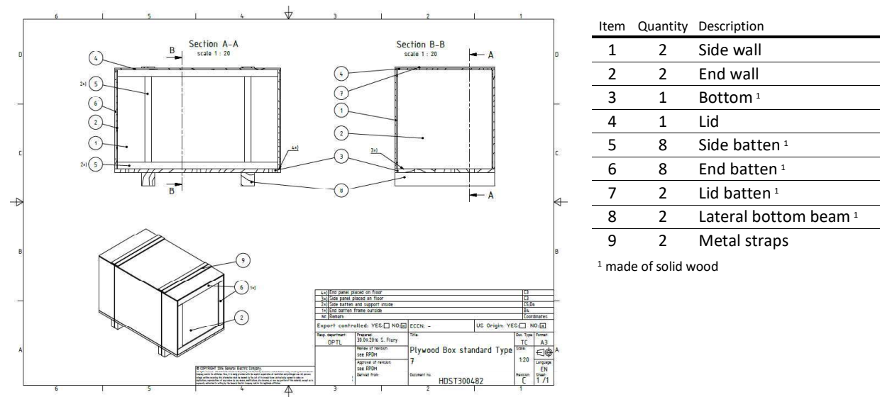
Figure 5: Plywood box type 7
