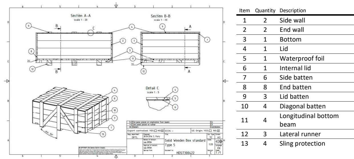
Figure 3: Solid wooden box type 5
