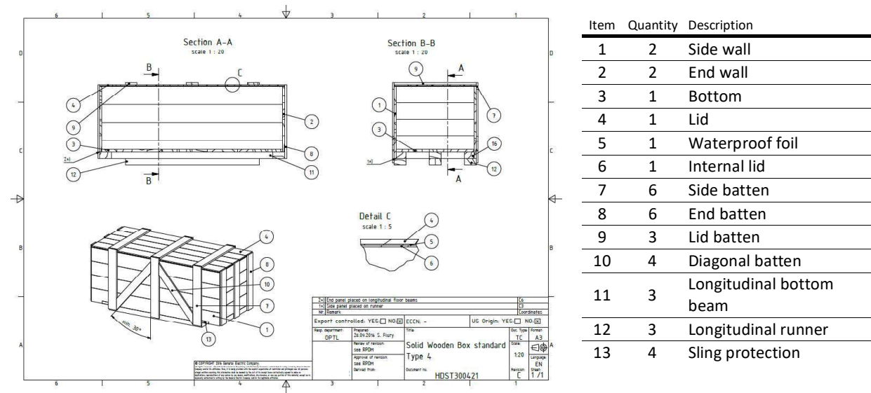
Figure 2: Solid wooden box type 4
