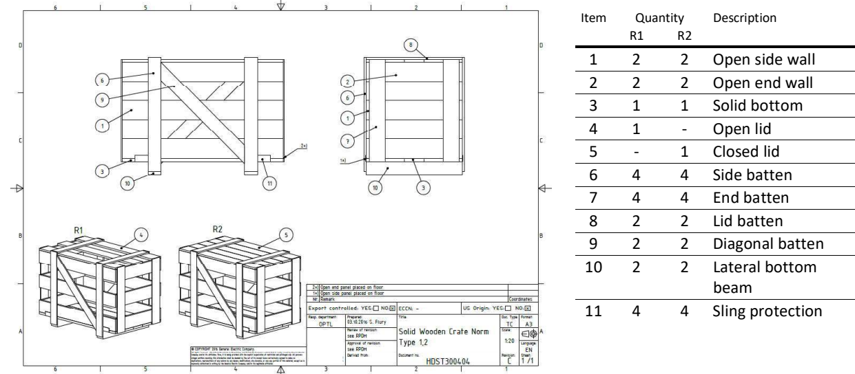
Figure 7: Solid wooden crate type 1 and 2
