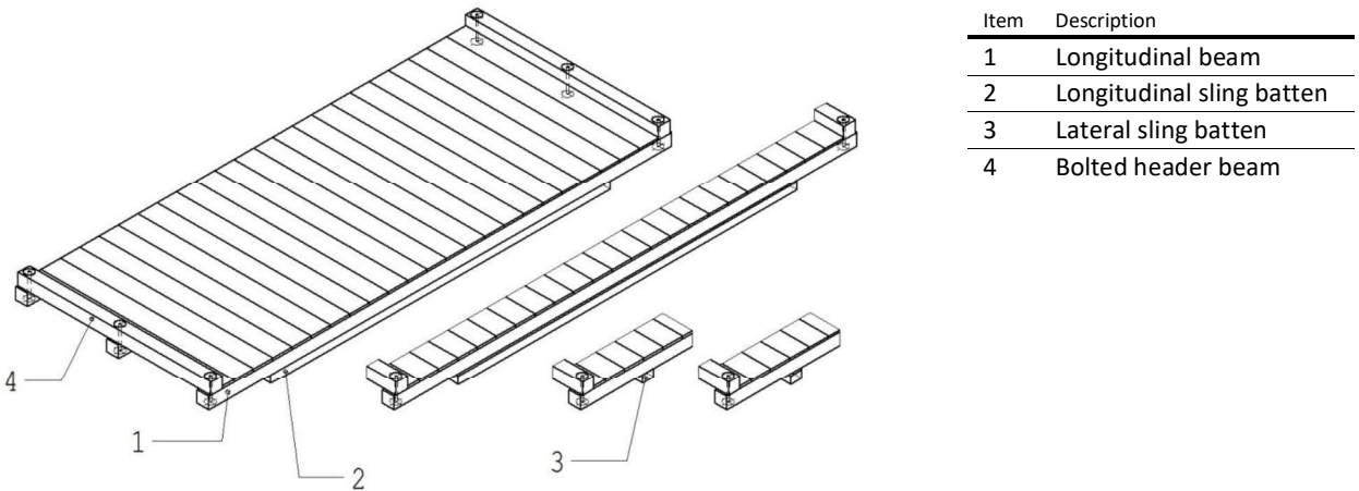
Figure 11: Bottom elements
