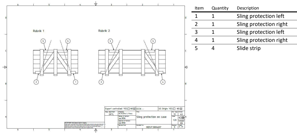
Figure 26: Fittings for box protection
