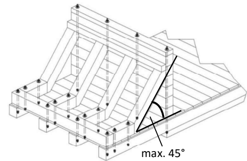
Figure 18: Maximum angle of supporting timbers
