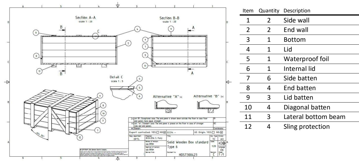
Figure 4: Solid wooden box type 6
