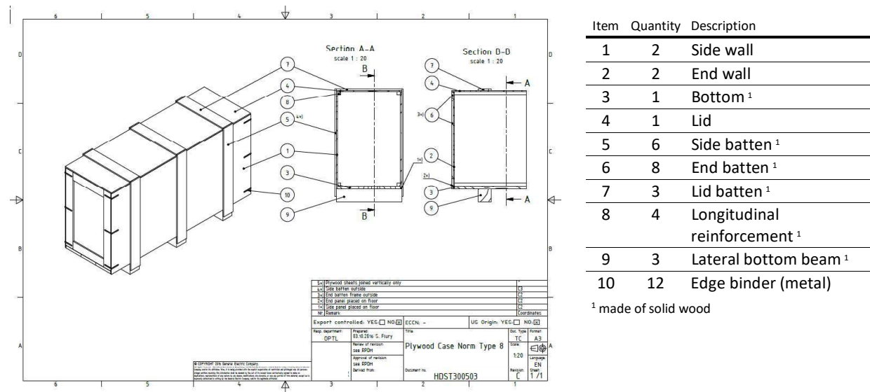
Figure 6: Plywood box type 8
