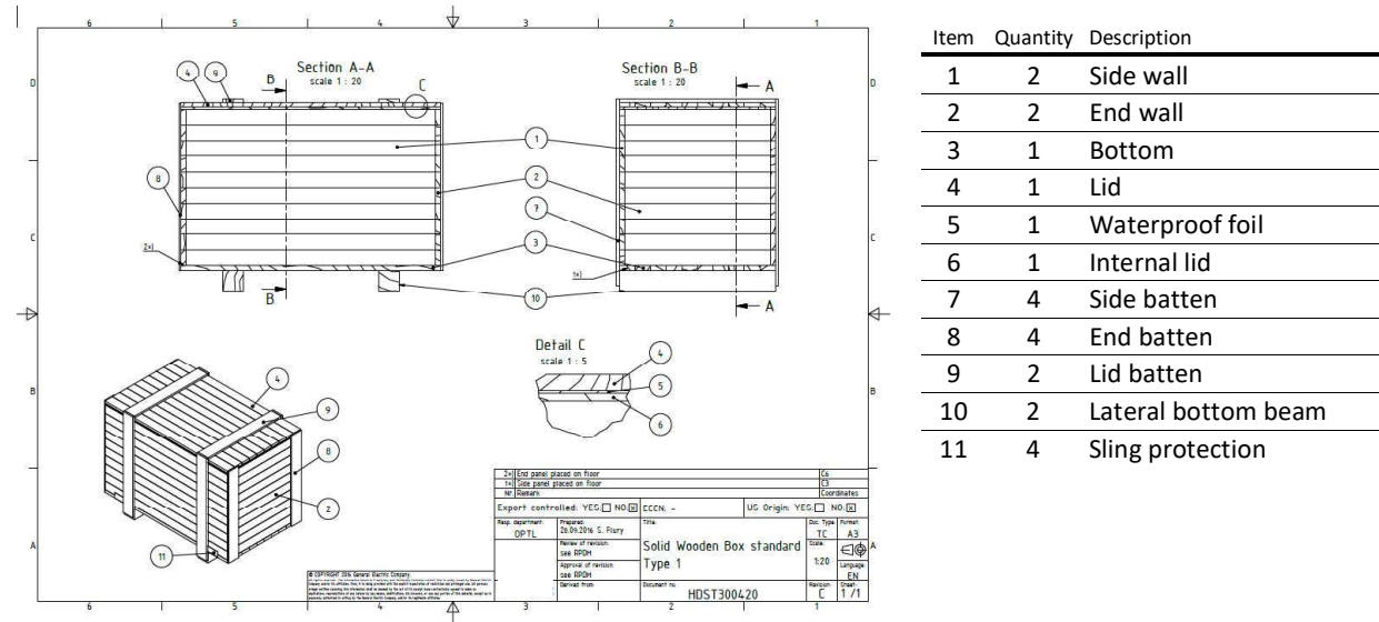
Figure 1: Solid wooden box type 1
