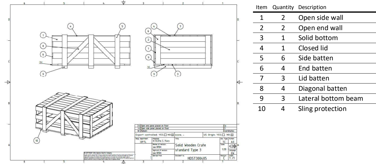
Figure 8: Solid wooden crate type 3
